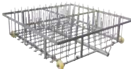
SH-55-140 Spindle Header (140 position bottle washing)
